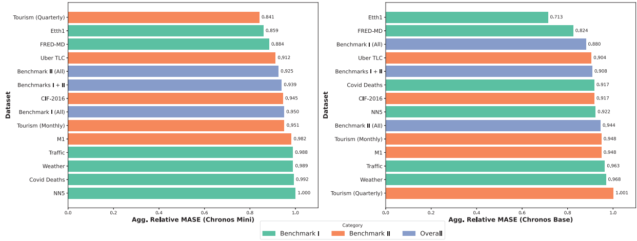
Figure 3: Aggregated Relative MASE performance for Chronos Mini and Chronos Base across datasets and benchmarks.
